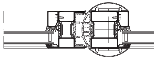
Fingerschutztür Porte anti-pince doigts Anti-finger trap door
