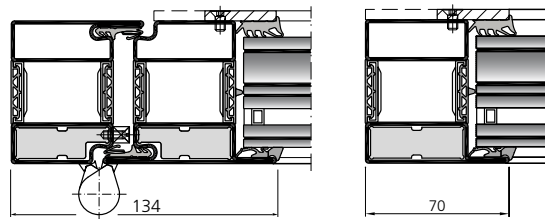
Fenster, Tür durchschusshemmend FB4NS Fenêtre, porte pare-balles FB4NS Bullet proof door and window FB4NS
